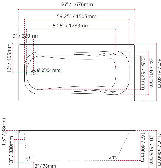
MODEL NUMBER : 4261 (LEFT HAND DRAIN LOCATION)
