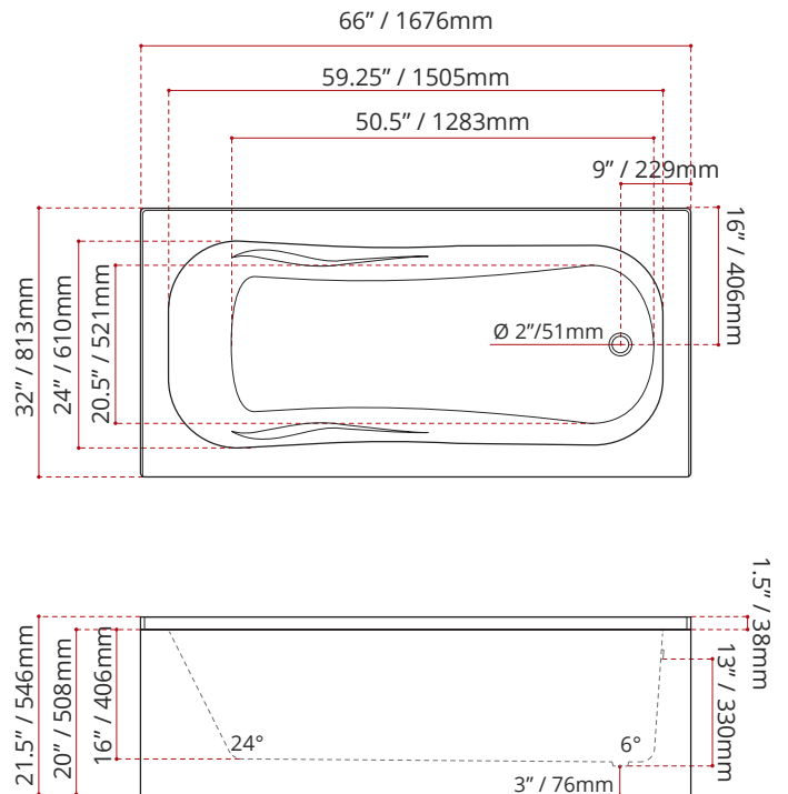
MODEL NUMBER : 4271 (RIGHT HAND DRAIN LOCATION)
