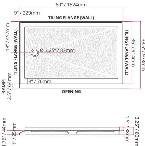
BSSTOD6036L1 (LEFT HAND DRAIN LOCATION)
