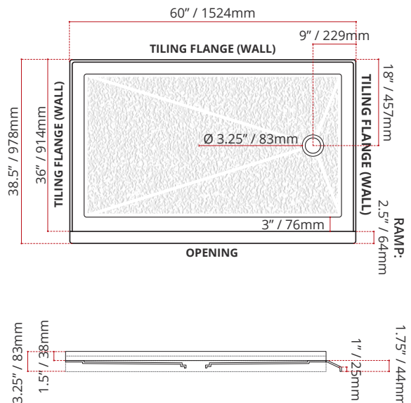
BSSTOD6036R1 (RIGHT HAND DRAIN LOCATION)
