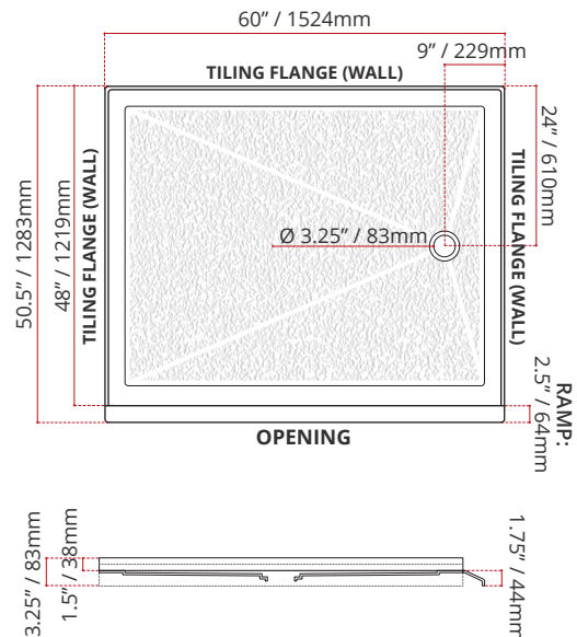
BSSTOD6048R1 (RIGHT HAND DRAIN LOCATION)
