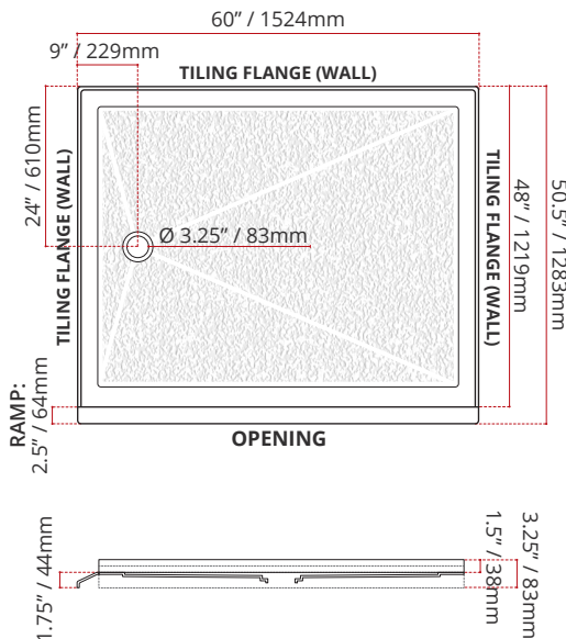
BSSTOD6048L1 (LEFT HAND DRAIN LOCATION)
