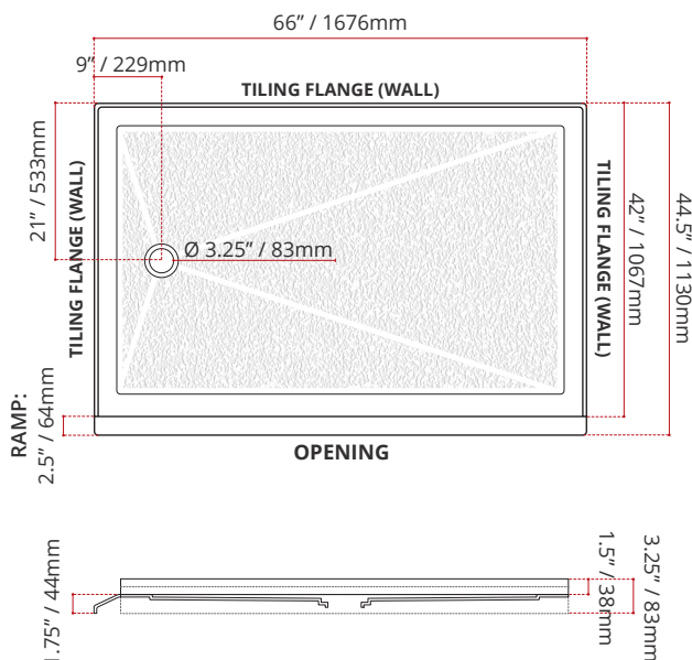
BSSTOD6642L1 (LEFT HAND DRAIN LOCATION)
