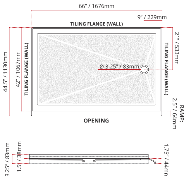
BSSTOD6642R1 (RIGHT HAND DRAIN LOCATION)
