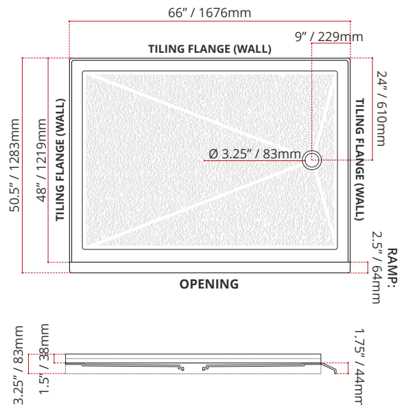
BSSTOD6648R1 (RIGHT HAND DRAIN LOCATION)
