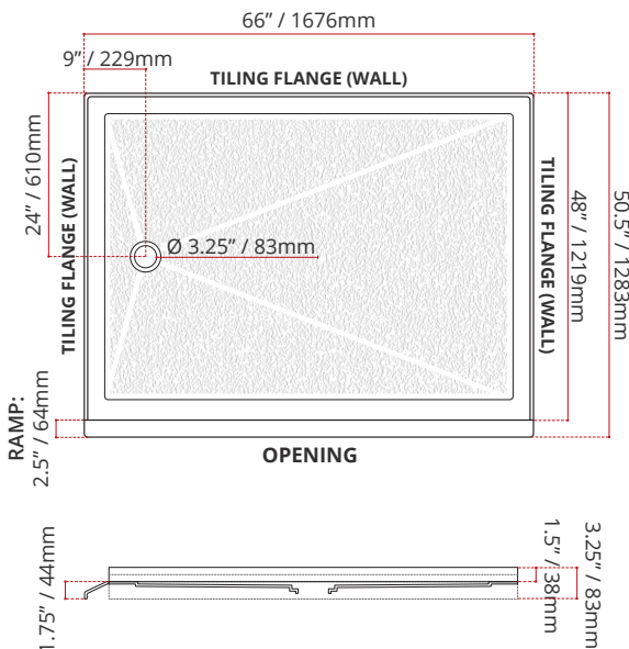
BSSTOD6648L1 (LEFT HAND DRAIN LOCATION)
