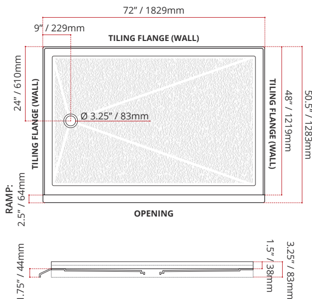
BSSTOD7248L1 (LEFT HAND DRAIN LOCATION)
