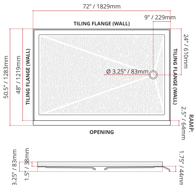
BSSTOD7248R1 (RIGHT HAND DRAIN LOCATION)
