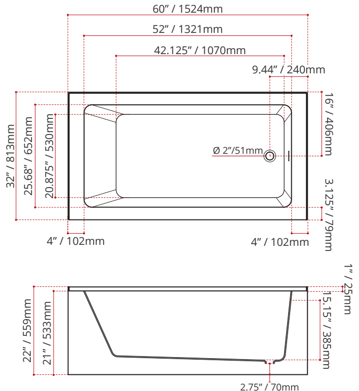
MODEL NUMBER : 2641 (RIGHT HAND DRAIN LOCATION)
