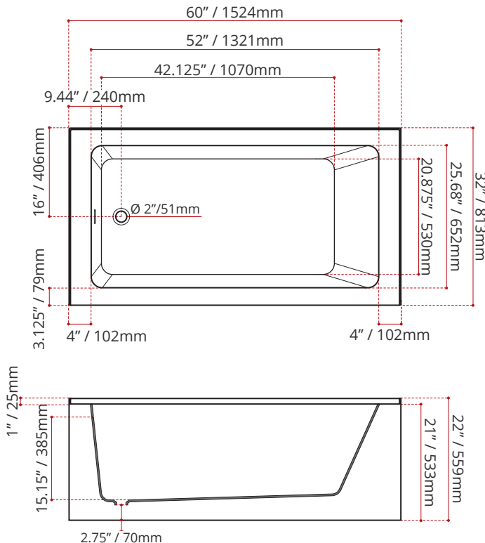
MODEL NUMBER : 2631 (LEFT HAND DRAIN LOCATION)
