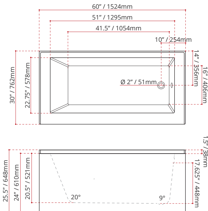
MODEL NUMBER : 1161 (RIGHT HAND DRAIN LOCATION)
