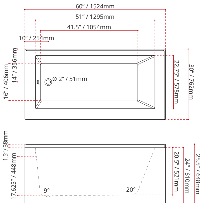
MODEL NUMBER : 1151 (LEFT HAND DRAIN LOCATION)
