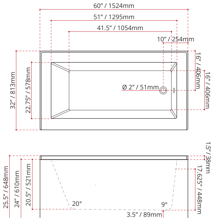
MODEL NUMBER : 1185 (RIGHT HAND DRAIN LOCATION)
