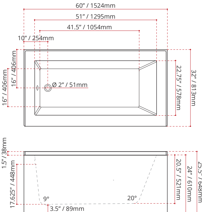
MODEL NUMBER : 1175 (LEFT HAND DRAIN LOCATION)
