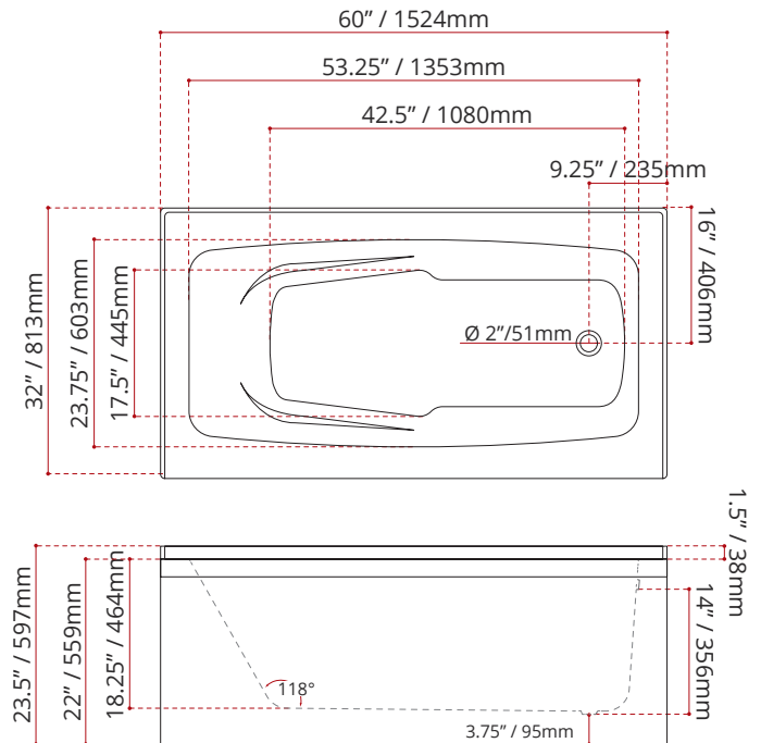
MODEL NUMBER : 5231 (RIGHT HAND DRAIN LOCATION)
