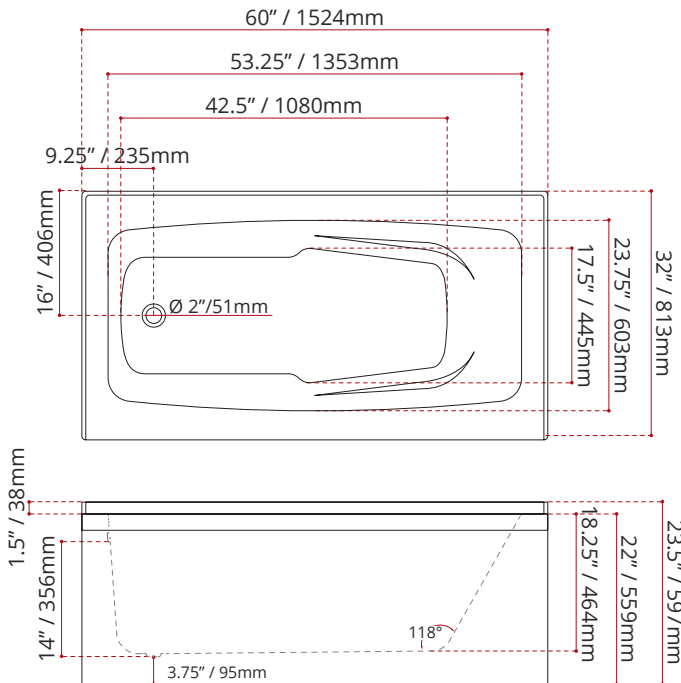
MODEL NUMBER : 5221 (LEFT HAND DRAIN LOCATION)
