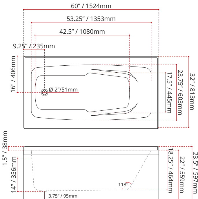
MODEL NUMBER : 5225 (LEFT HAND DRAIN LOCATION)
