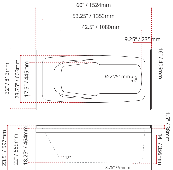
MODEL NUMBER : 5235 (RIGHT HAND DRAIN LOCATION)
