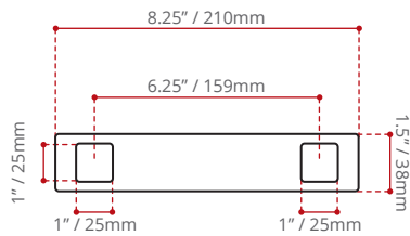
TOILET SEAT BRACKET
