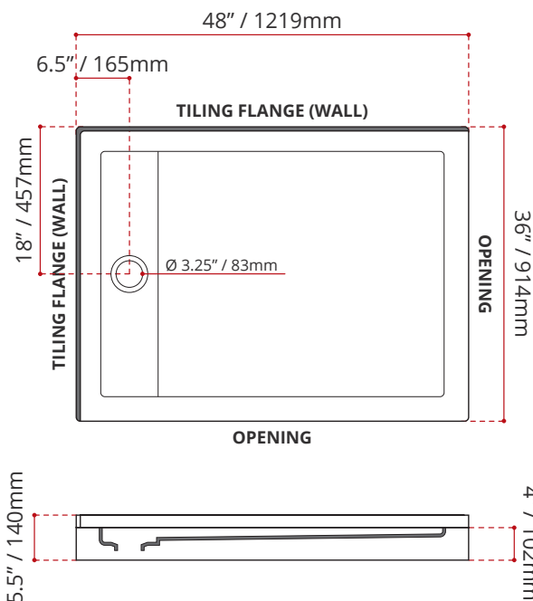
SDTLD4836L4 (LEFT HAND DRAIN LOCATION) (RIGHT HAND THRESHOLD / OPENING)
