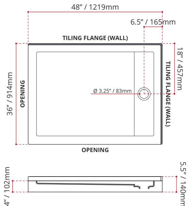
SDTLD4836R4 (RIGHT HAND DRAIN LOCATION) (LEFT HAND THRESHOLD / OPENING)
