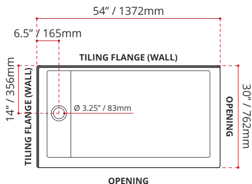
SDTLD5430L1 (LEFT HAND DRAIN LOCATION) (RIGHT HAND THRESHOLD / OPENING)
