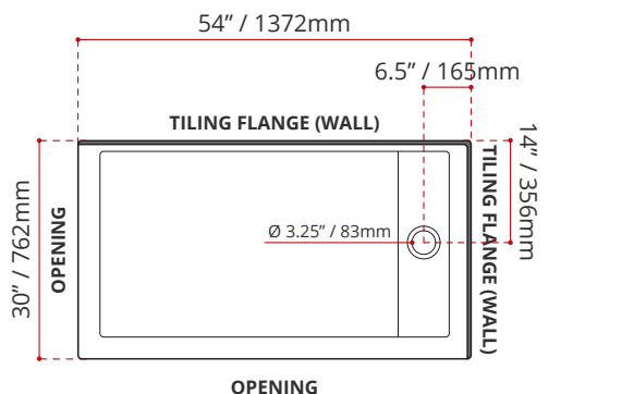
SDTLD5430R1 (RIGHT HAND DRAIN LOCATION) (LEFT HAND THRESHOLD / OPENING)
