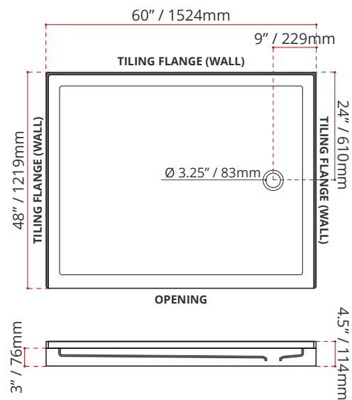
SSTOD6048R1 (RIGHT HAND DRAIN LOCATION)
