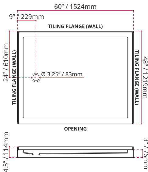
SSTOD6048L1 (LEFT HAND DRAIN LOCATION)
