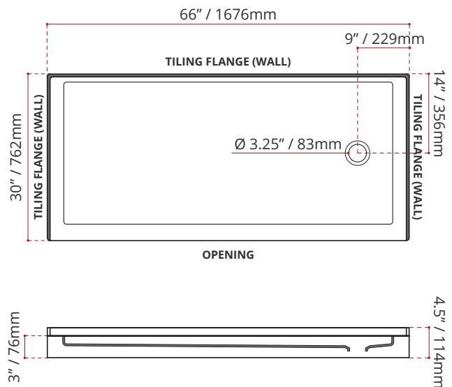
SSTOD6630R1 (RIGHT HAND DRAIN LOCATION)
