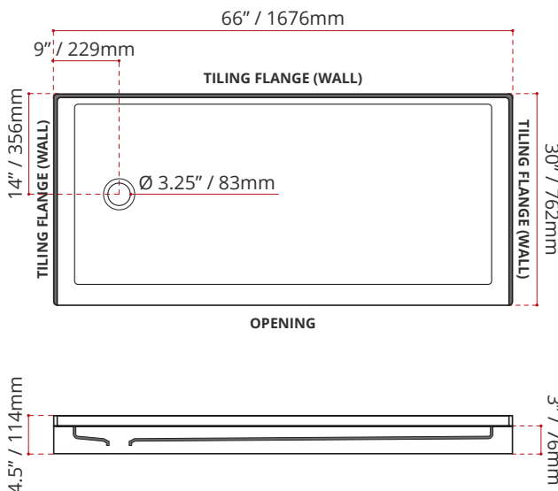
SSTOD6630L1 (LEFT HAND DRAIN LOCATION)
