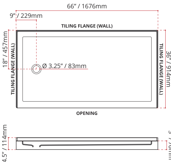
SSTOD6636L1 (LEFT HAND DRAIN LOCATION)
