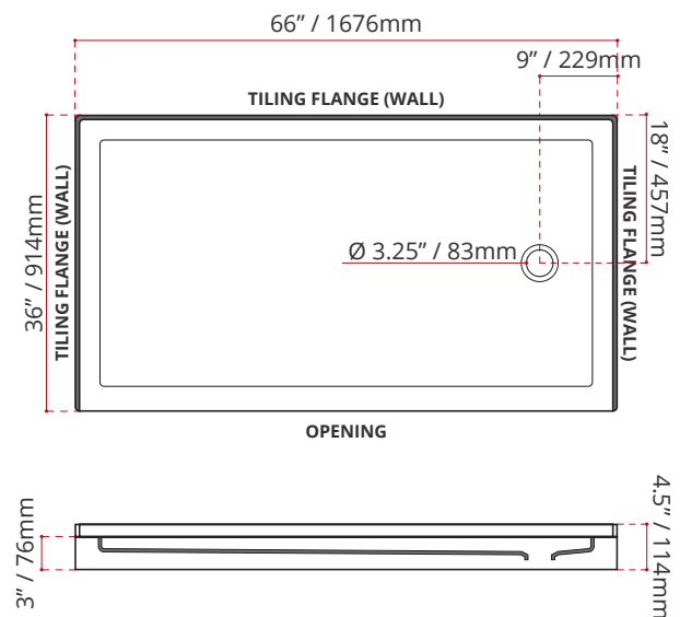
SSTOD6636R1 (RIGHT HAND DRAIN LOCATION)
