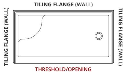
RIGHT HAND DRAIN LOCATION - LEFT HAND SEAT
